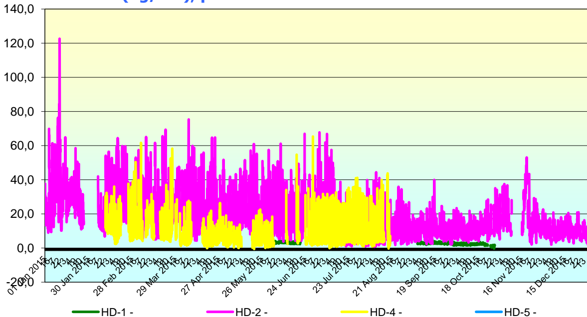
Channel: \text{NO}_2 ( \mu\text{g}/\text{m}^3 ), period: 01 Jan 2015-31 Dec 2015 - Validate data
